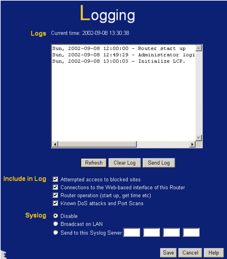
Figure 41: Logs Screen
